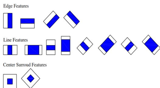
Gambar 1 Haar-like Feature.
