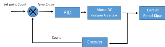
Gambar 10 Diagram Kendali
