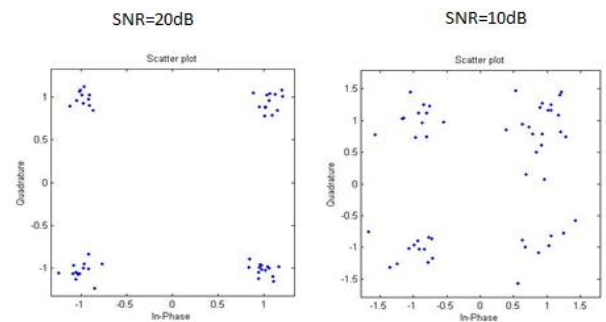
Gambar 7: Scatter diagram QAM-4 plus noise
