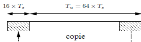
Gambar 10: Cyclic Prefix
