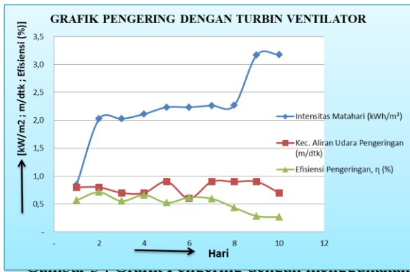
Turbin Ventilator
