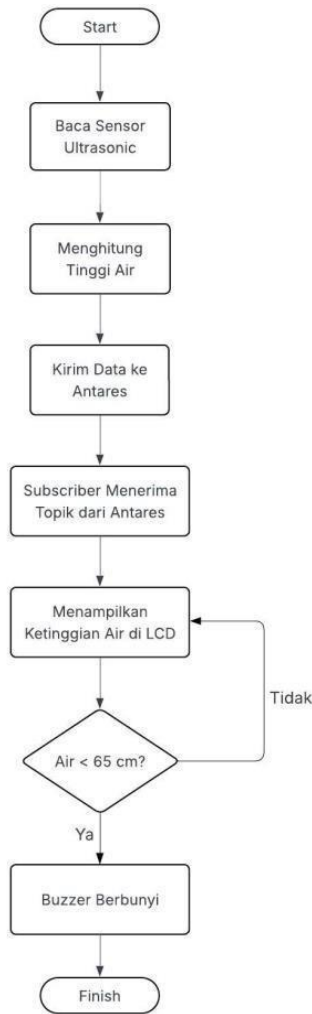
Figure 3. Software Design Flowchart
