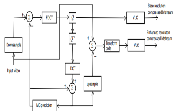
Gambar2. Spatial Scalability
