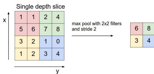
Gambar 5. Max Pooling
