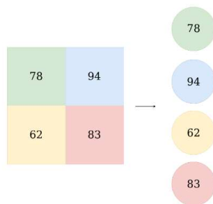
Gambar 6. Flatening
